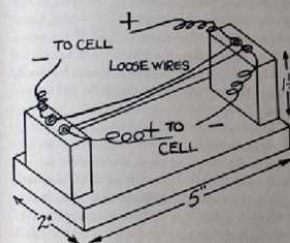
Fig. 1. Wires carrying electricity act in the manner of magnets. Electricity passing in the same direction in both causes repulsion. When passing in opposite directions, attraction between the wires is noticed.
