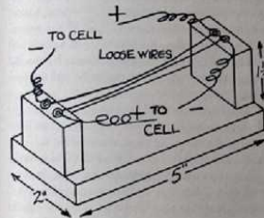
Fig. 4. Wires carrying electricity act in the manner of magnets. Electricity passing in the same direction in both causes repulsion. When passing in opposite directions, attraction between the wires is noticed.
